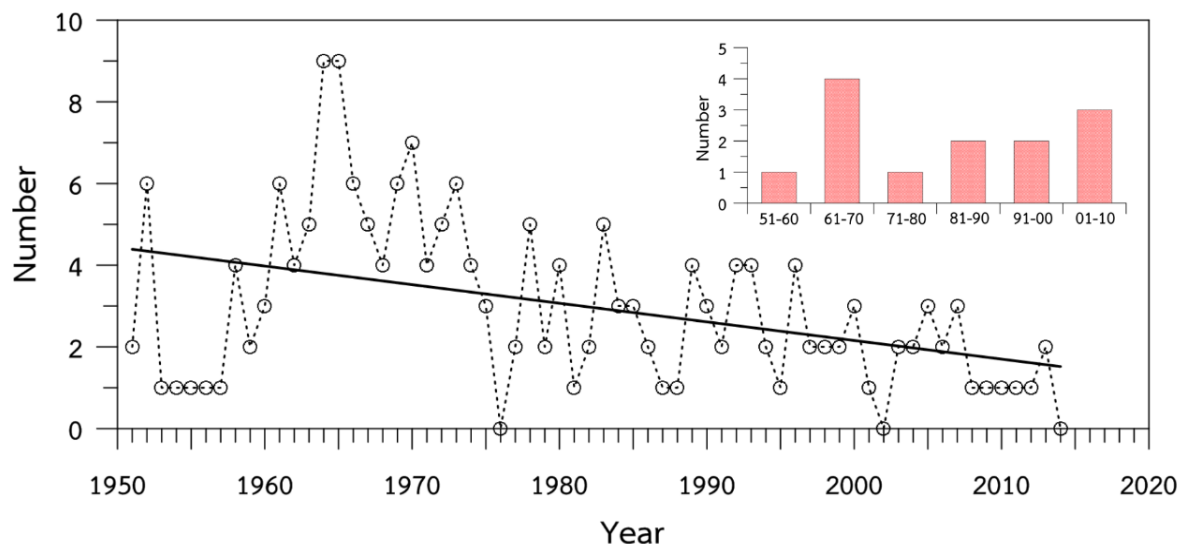
Figure 3 Frequency of tropical cyclones (depression, tropical storm and typhoon) entering Thailand during 1951-2014. The small picture inserted shows averaged frequency of tropical storm and typhoon occurred every ten year.
